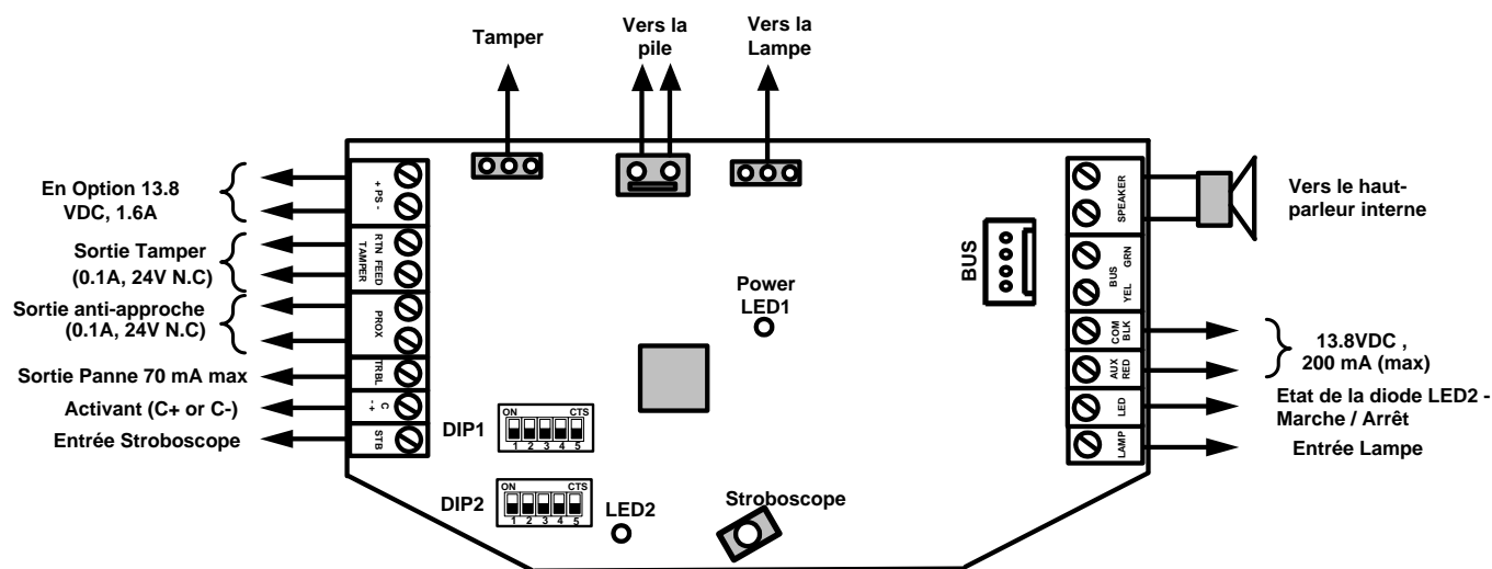
Figure 1 - Configuration autonome
